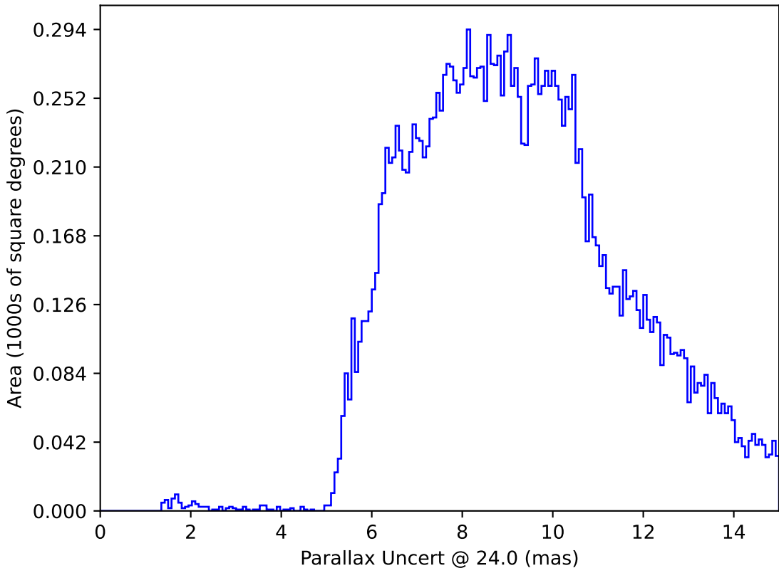
early_ss_template_fpextra1.5_v3.4_10yrs : Parallax Uncert @ 24.0
