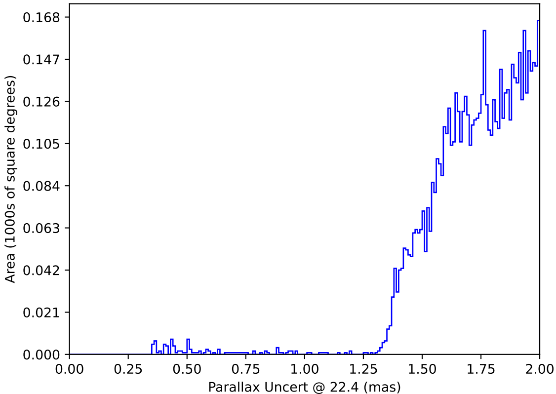
early_ss_template_fpextra1.5_v3.4_10yrs : Parallax Uncert @ 22.4
