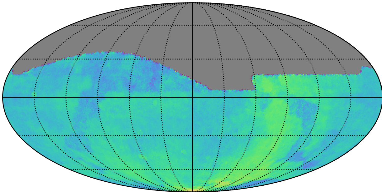
early_ss_template_fpextra1.5_v3.4_10yrs : Parallax Coverage @ 24.0
