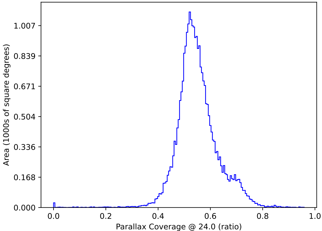
early_ss_template_fpextra1.5_v3.4_10yrs : Parallax Coverage @ 24.0
