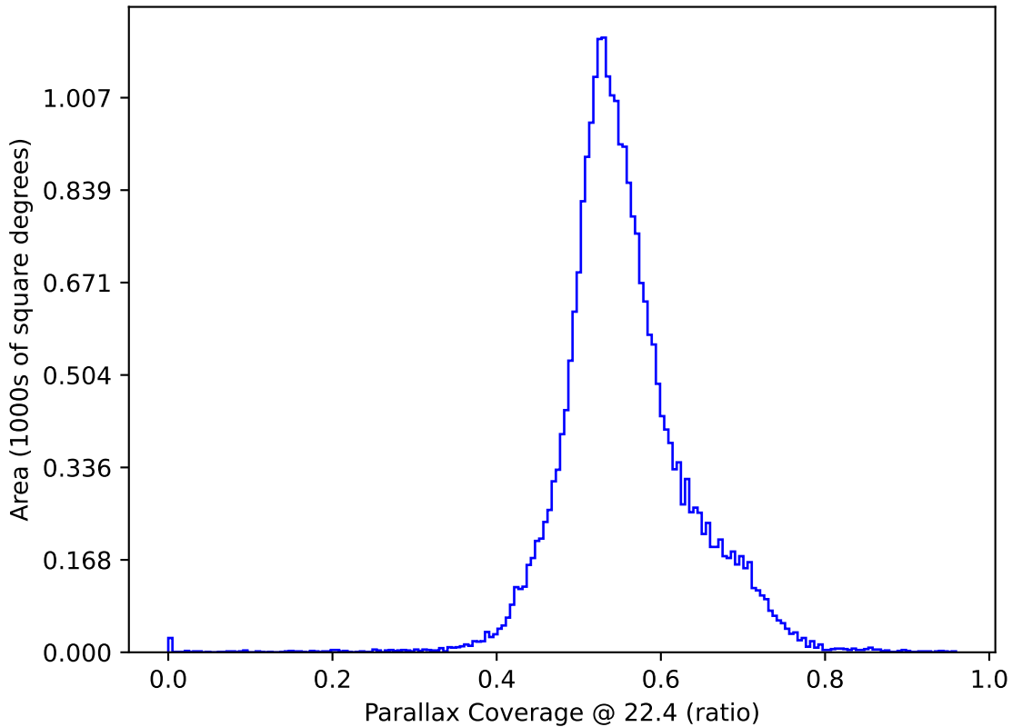
early_ss_template_fpextra1.5_v3.4_10yrs : Parallax Coverage @ 22.4
