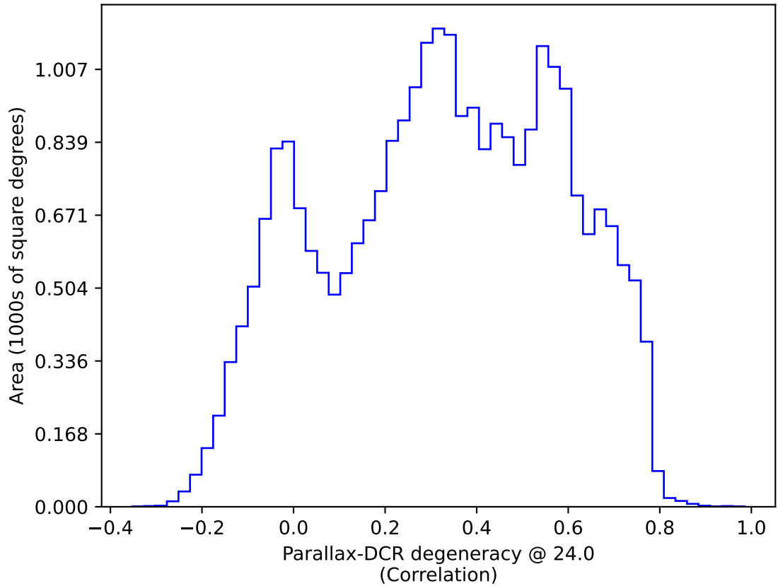
early_ss_template_fpextra1.5_v3.4_10yrs : Parallax-DCR degeneracy @ 24.0
