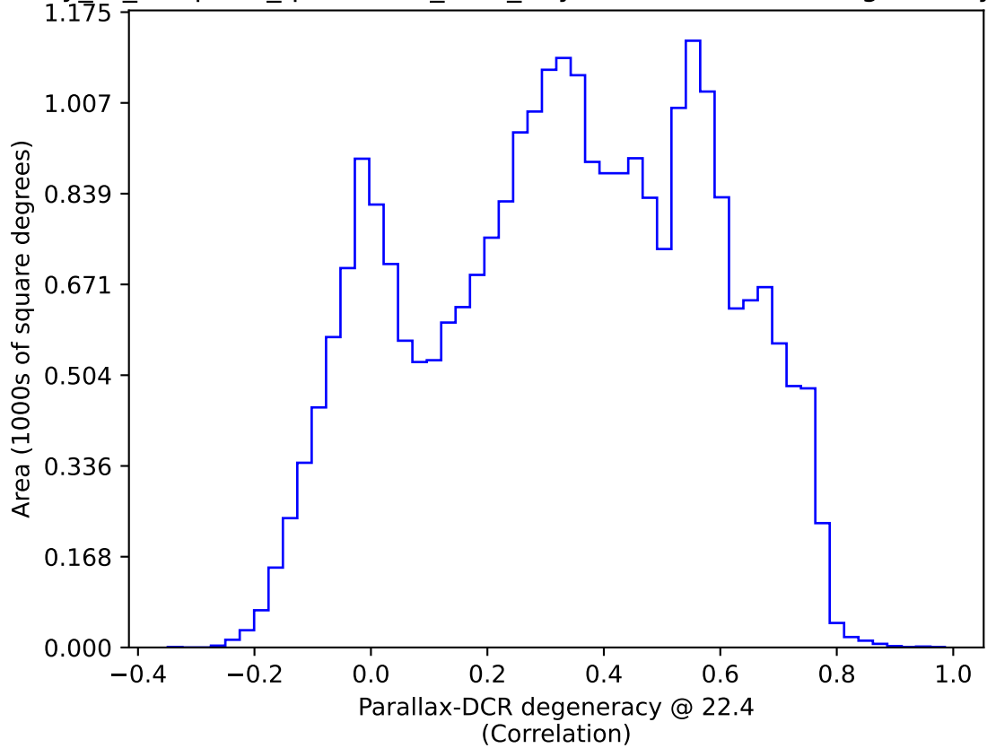
early_ss_template_fpextra1.5_v3.4_10yrs : Parallax-DCR degeneracy @ 22.4
