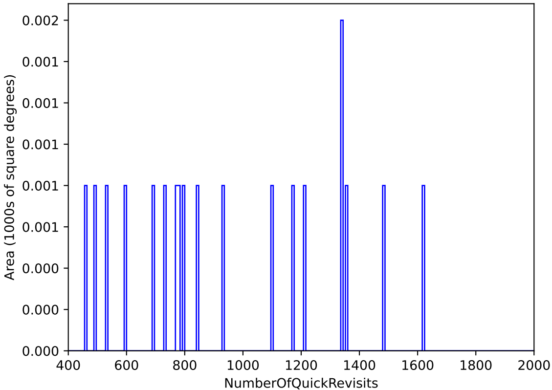
early_ss_template_fpextra1.5_v3.4_10yrs : NumberOfQuickRevisits
