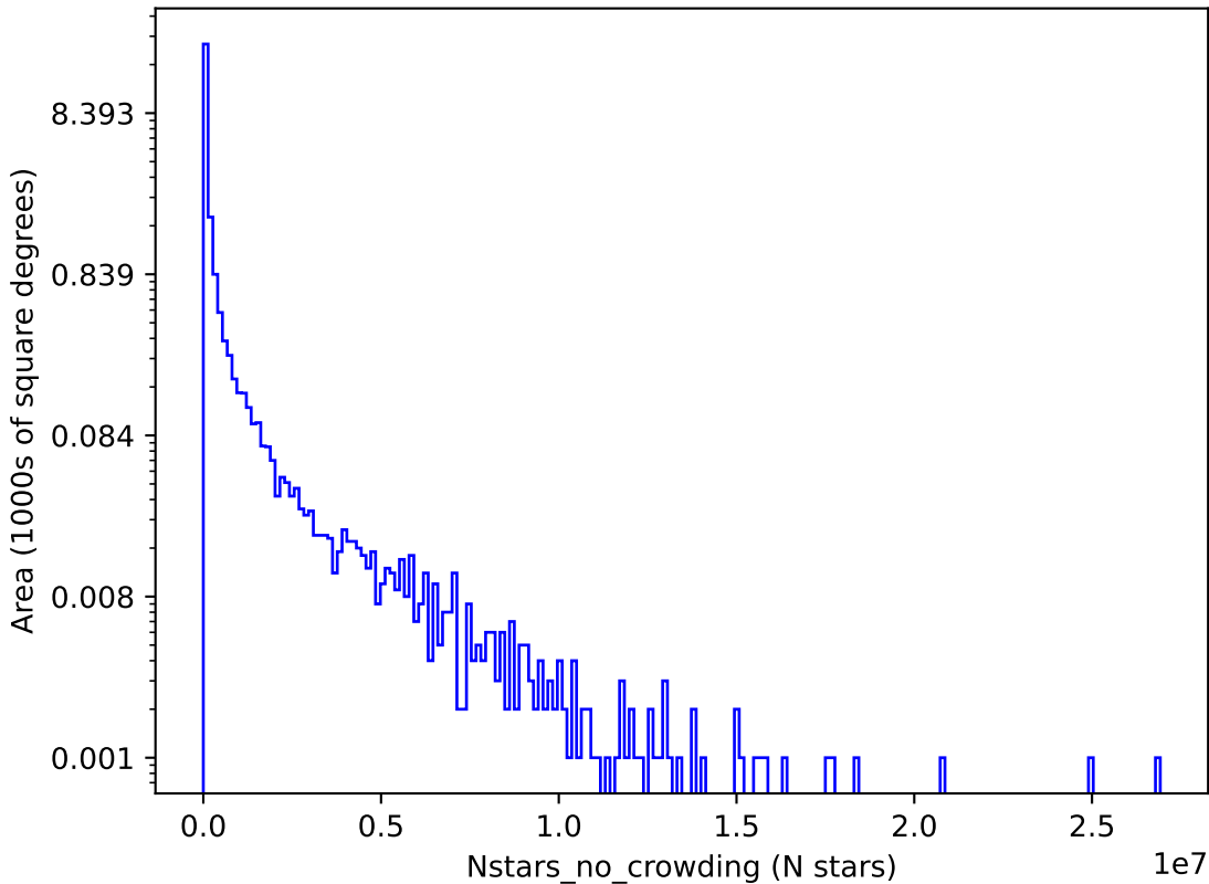
early_ss_template_fpextra1.5_v3.4_10yrs z: Nstars_no_crowding
