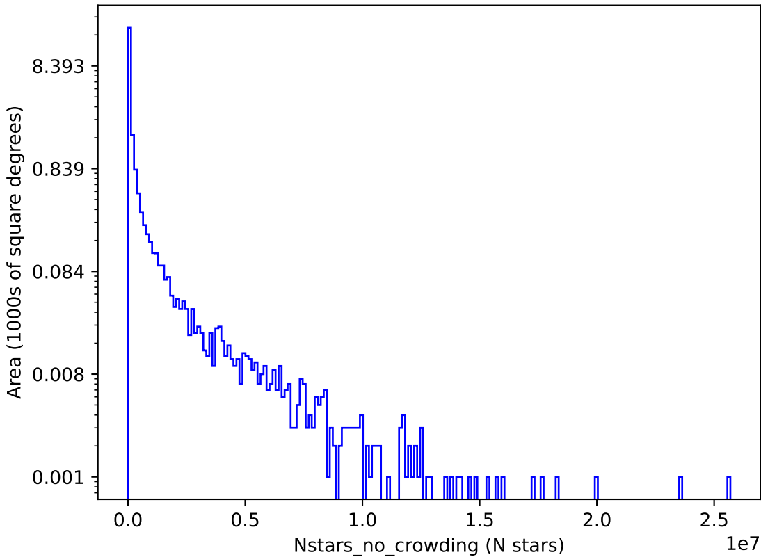
early_ss_template_fpextra1.5_v3.4_10yrs y: Nstars_no_crowding
