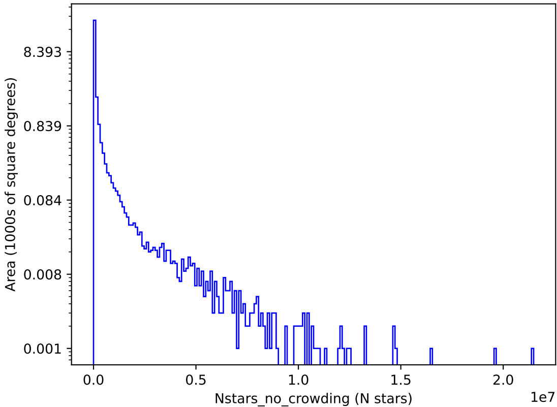
early_ss_template_fpextra1.5_v3.4_10yrs r: Nstars_no_crowding
