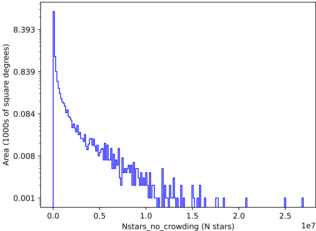
early_ss_template_fpextra1.5_v3.4_10yrs i: Nstars_no_crowding
