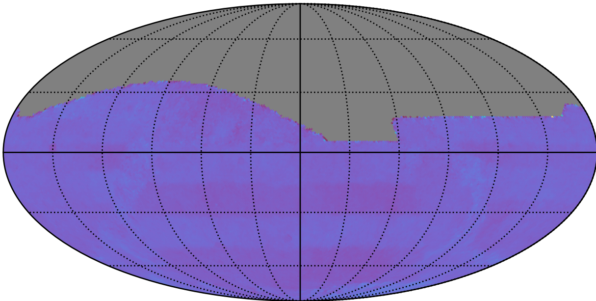
early_ss_template_fpextra1.5_v3.4_10yrs : Normalized Proper Motion Uncert @ 24.0
