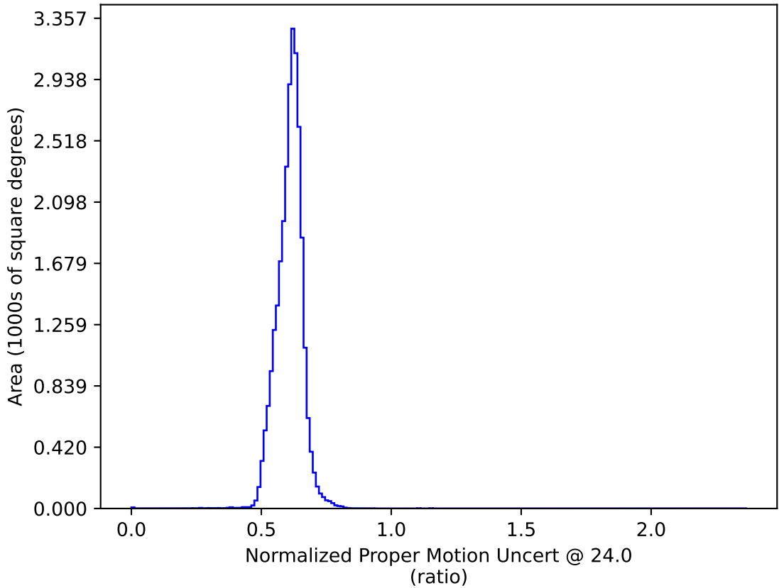
early_ss_template_fpextra1.5_v3.4_10yrs : Normalized Proper Motion Uncert @ 24.0
