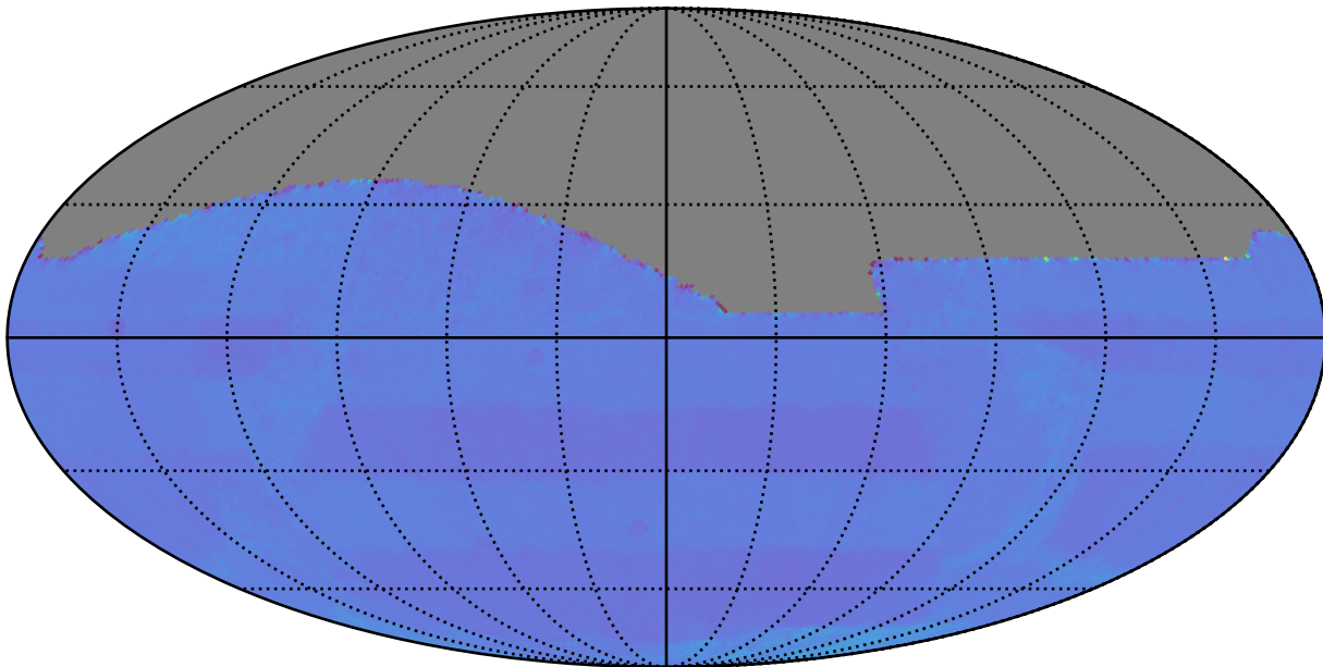
early_ss_template_fpextra1.5_v3.4_10yrs : Normalized Proper Motion Uncert @ 20.5
