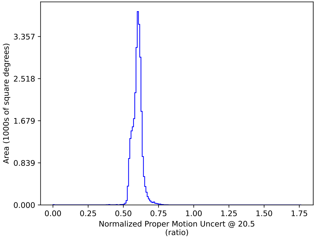
early_ss_template_fpextra1.5_v3.4_10yrs : Normalized Proper Motion Uncert @ 20.5
