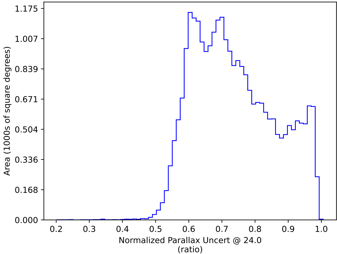
early_ss_template_fpextra1.5_v3.4_10yrs : Normalized Parallax Uncert @ 24.0
