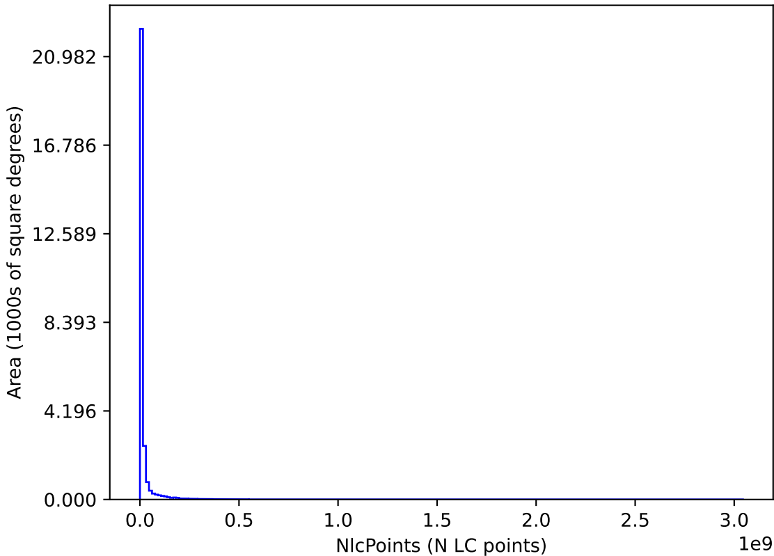
early_ss_template_fpextra1.5_v3.4_10yrs : NlcPoints
