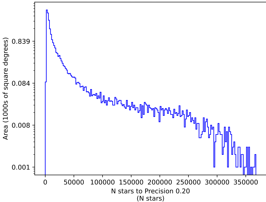
early_ss_template_fpextra1.5_v3.4_10yrs u: N stars to Precision 0.20
