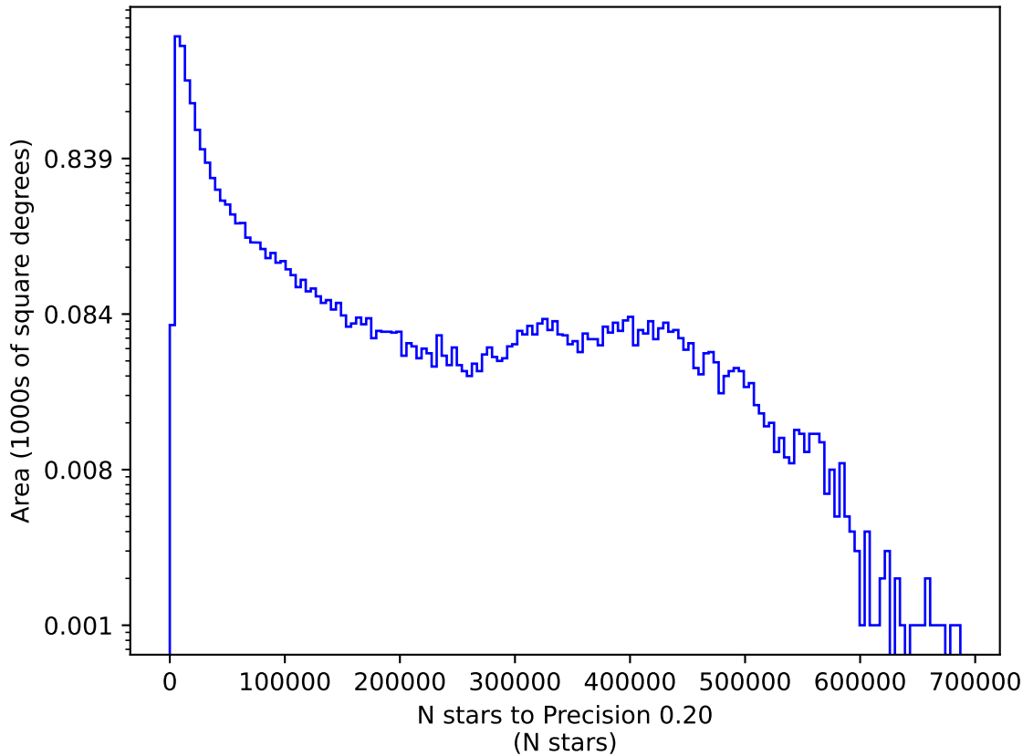
early_ss_template_fpextra1.5_v3.4_10yrs r: N stars to Precision 0.20
