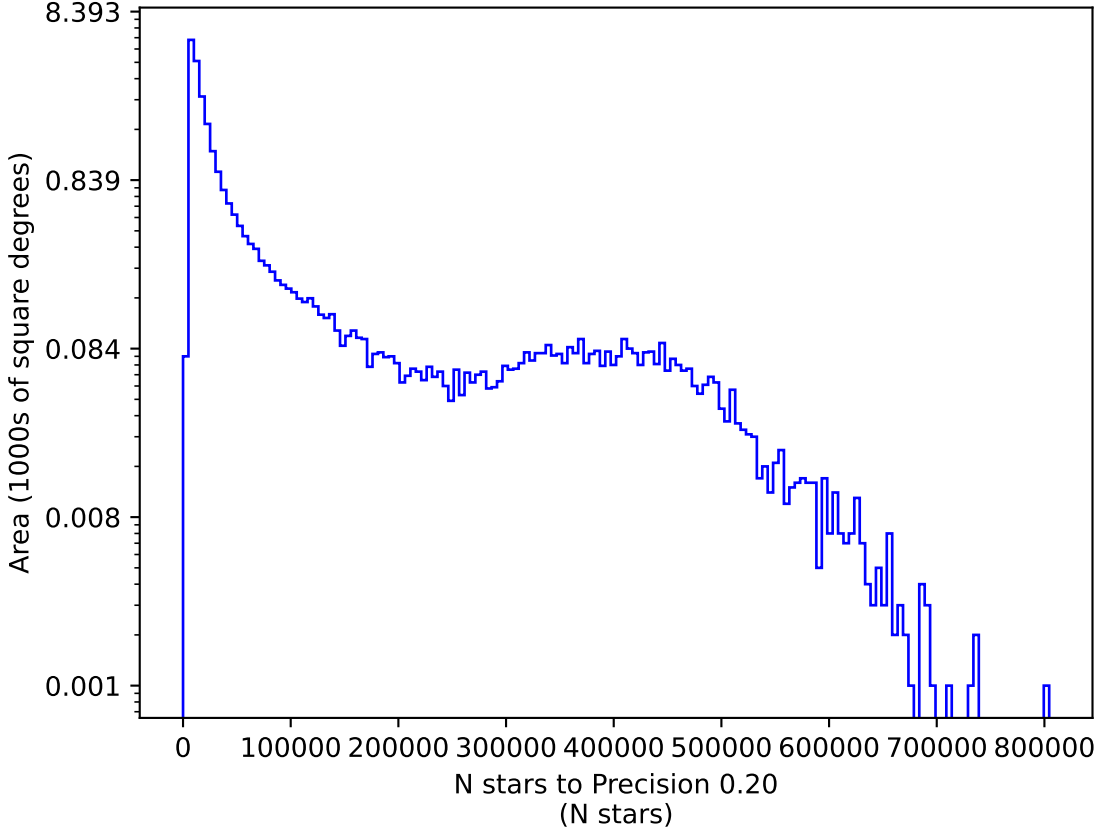
early_ss_template_fpextra1.5_v3.4_10yrs i: N stars to Precision 0.20
