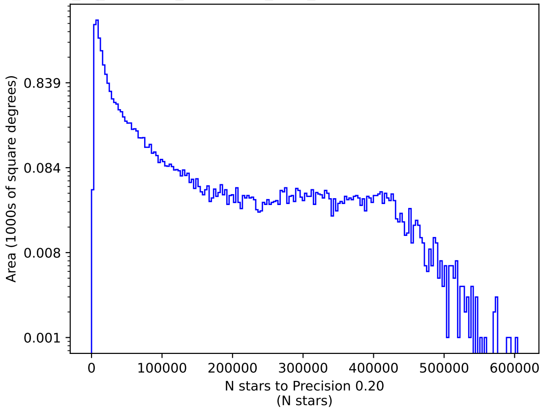
early_ss_template_fpextra1.5_v3.4_10yrs g: N stars to Precision 0.20
