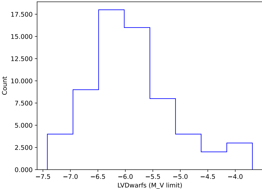
early_ss_template_fpextra1.5_v3.4_10yrs gi: LVDwarfs
