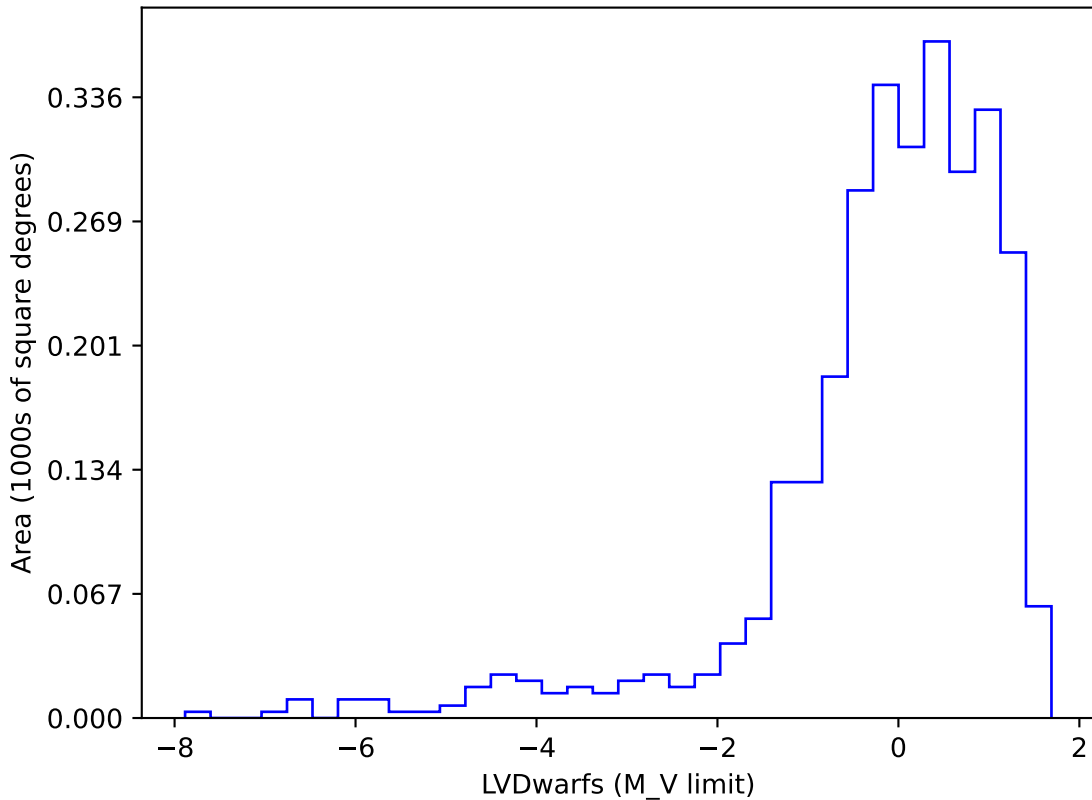
early_ss_template_fpextra1.5_v3.4_10yrs gi SCP: LVDwarfs
