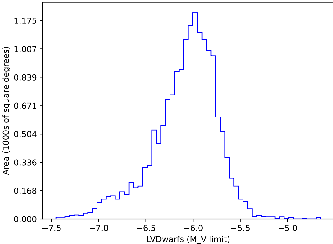
early_ss_template_fpextra1.5_v3.4_10yrs gi: LVDwarfs
