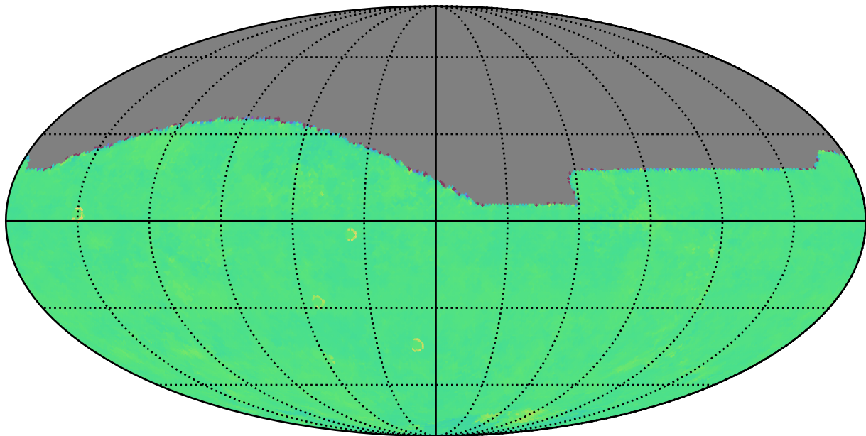
early_ss_template_fpextra1.5_v3.4_10yrs z: Kuiper rotTelPos
