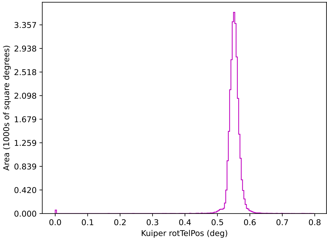
early_ss_template_fpextra1.5_v3.4_10yrs z: Kuiper rotTelPos
