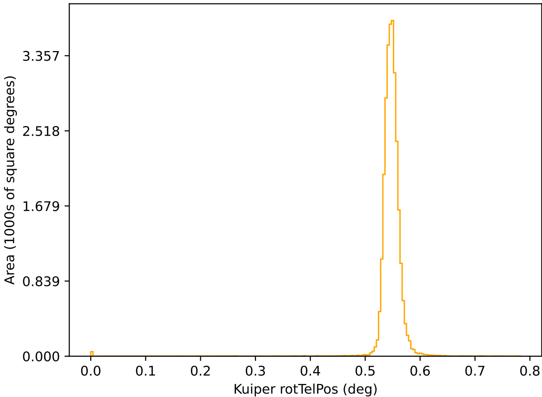
early_ss_template_fpextra1.5_v3.4_10yrs r: Kuiper rotTelPos
