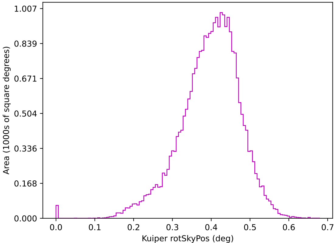
early_ss_template_fpextra1.5_v3.4_10yrs z: Kuiper rotSkyPos
