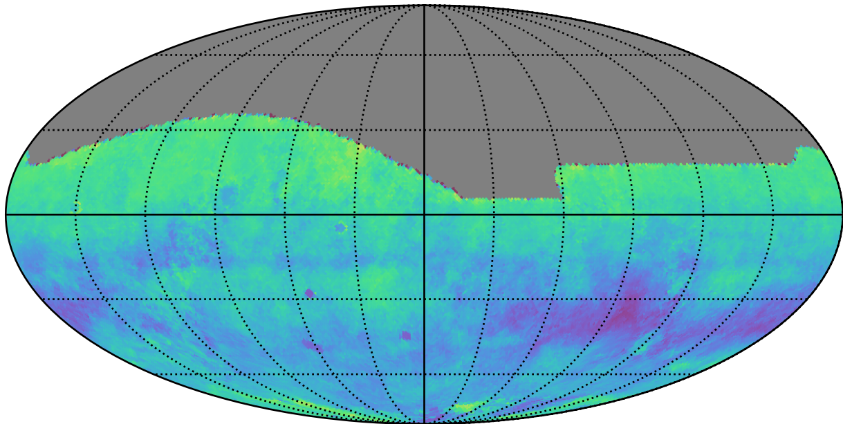
early_ss_template_fpextra1.5_v3.4_10yrs r: Kuiper rotSkyPos
