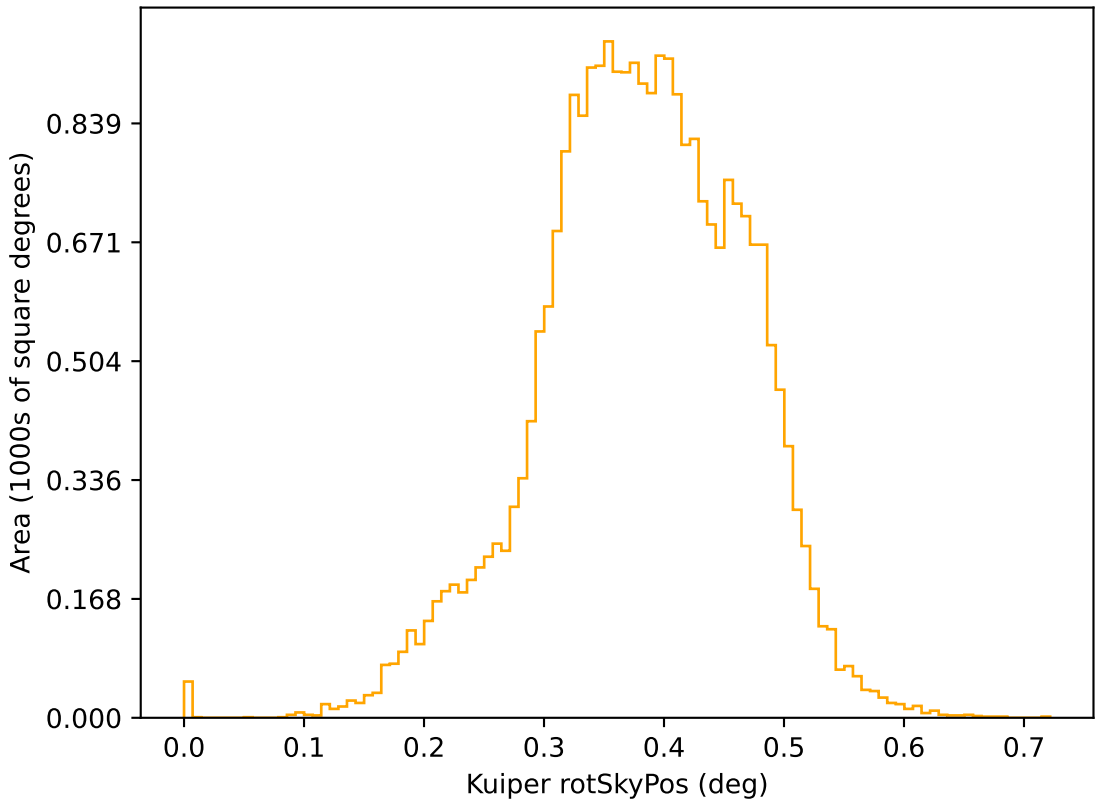
early_ss_template_fpextra1.5_v3.4_10yrs r: Kuiper rotSkyPos
