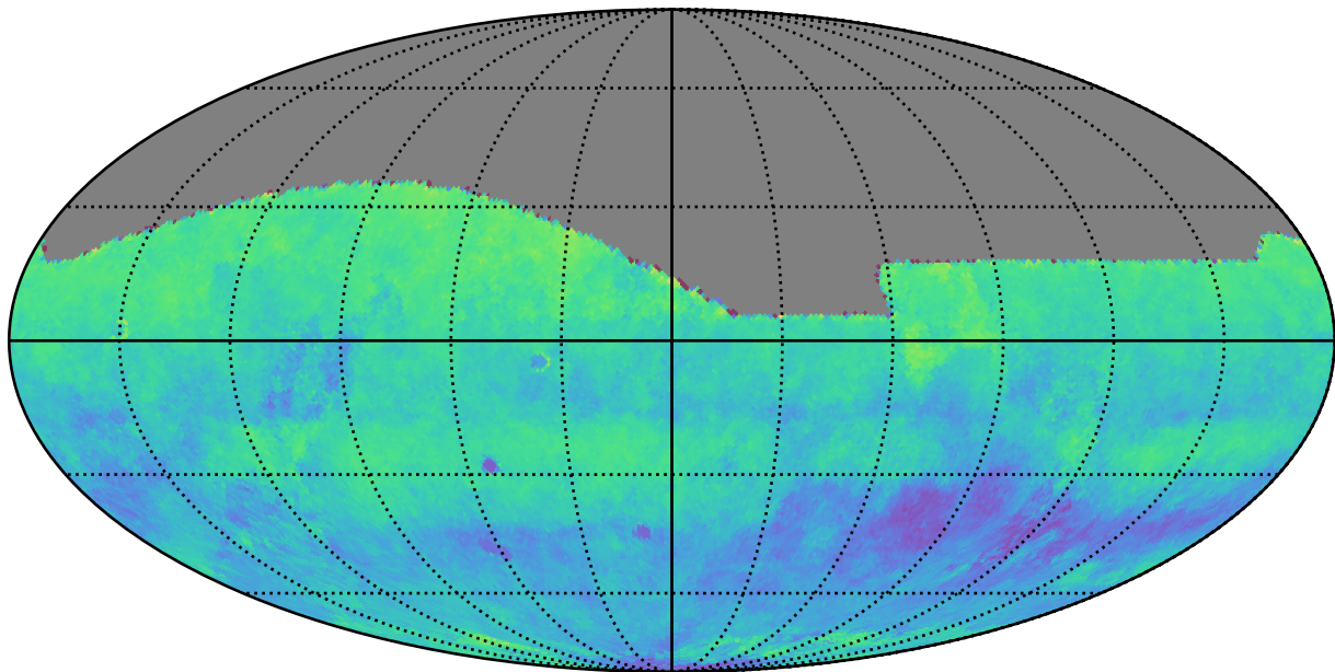
early_ss_template_fpextra1.5_v3.4_10yrs i: Kuiper rotSkyPos
