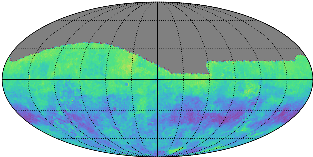
early_ss_template_fpextra1.5_v3.4_10yrs g: Kuiper rotSkyPos
