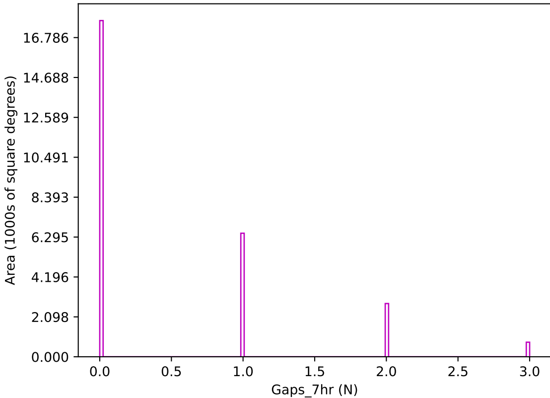
early_ss_template_fpextra1.5_v3.4_10yrs z band: Gaps_7hr
