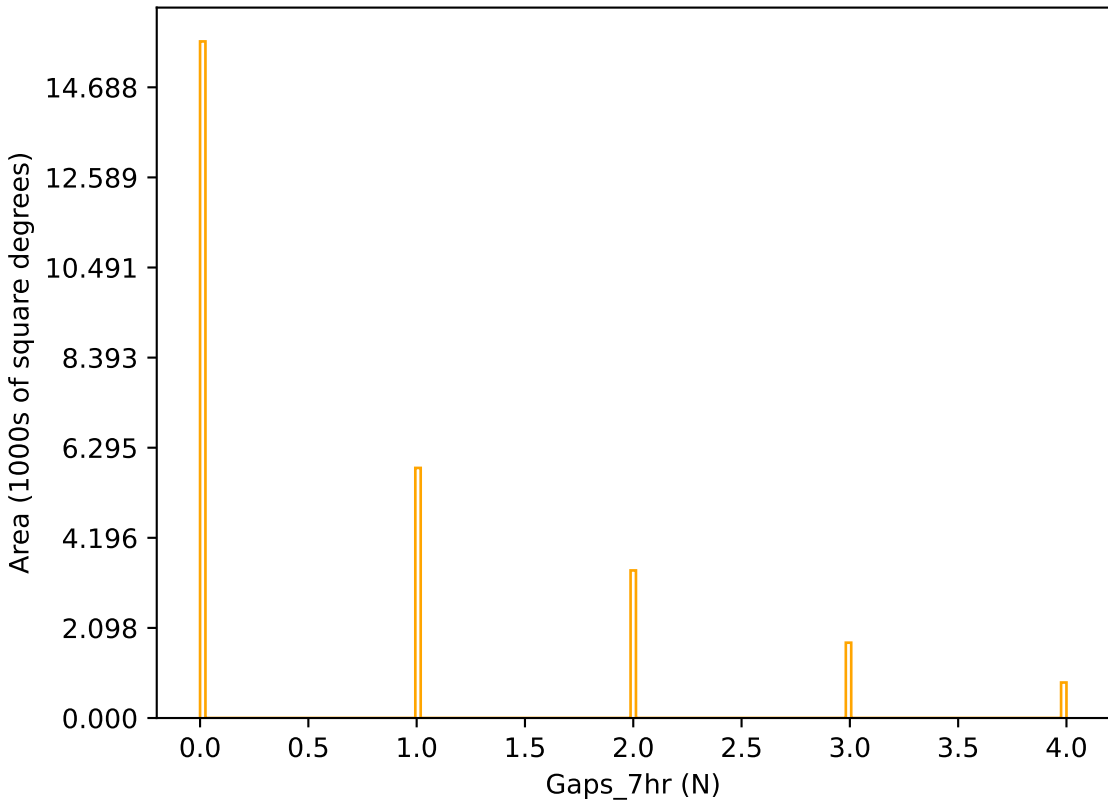
early_ss_template_fpextra1.5_v3.4_10yrs r band: Gaps_7hr
