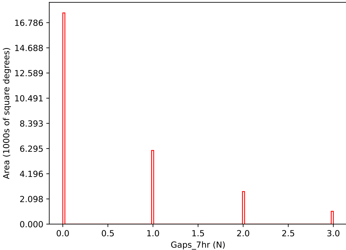
early_ss_template_fpextra1.5_v3.4_10yrs i band: Gaps_7hr
