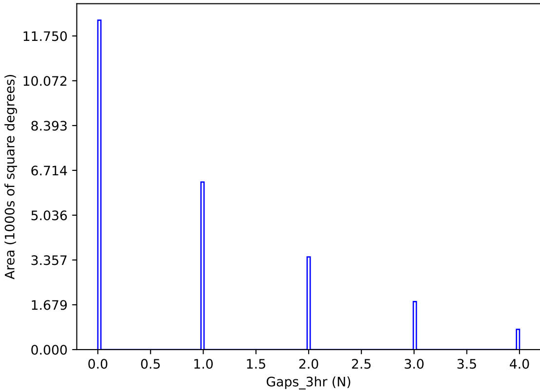
early_ss_template_fpextra1.5_v3.4_10yrs y band: Gaps_3hr
