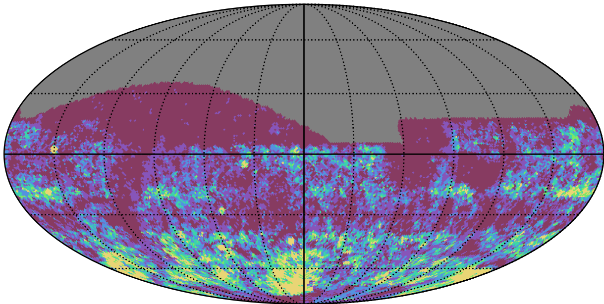
early_ss_template_fpextra1.5_v3.4_10yrs r band: Gaps_3hr
