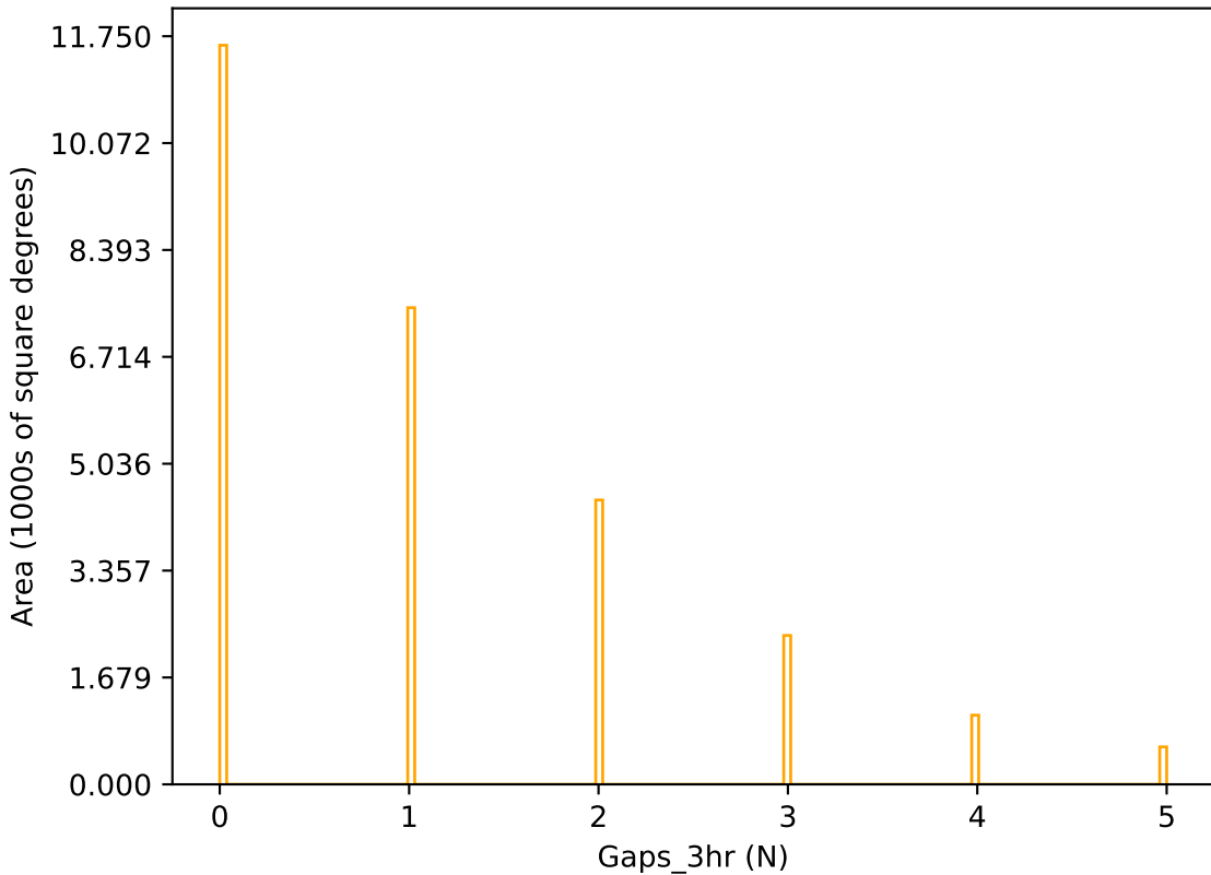
early_ss_template_fpextra1.5_v3.4_10yrs r band: Gaps_3hr
