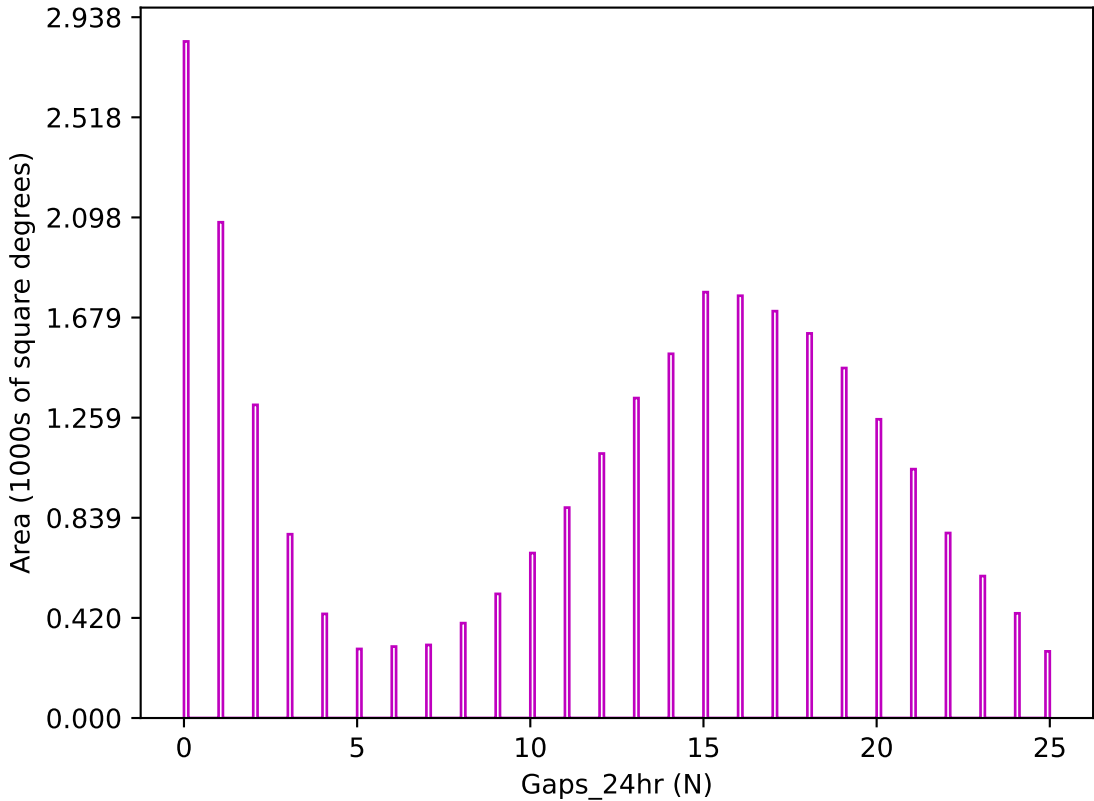
early_ss_template_fpextra1.5_v3.4_10yrs z band: Gaps_24hr
