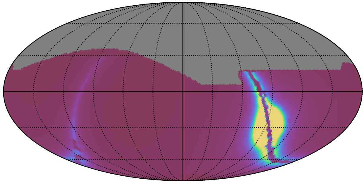
early_ss_template_fpextra1.5_v3.4_10yrs : GalplaneFootprintMetric_xray_binaries_map_Tau_73_0
