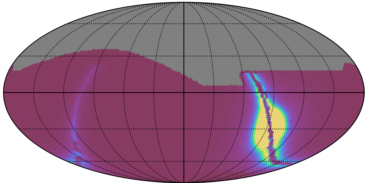
early_ss_template_fpextra1.5_v3.4_10yrs : GalplaneFootprintMetric_xray_binaries_map_Tau_46_5
