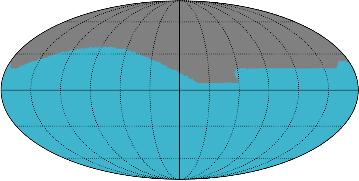
early_ss_template_fpextra1.5_v3.4_10yrs : GalplaneFootprintMetric_xray_binaries_map_Tau_2_0
