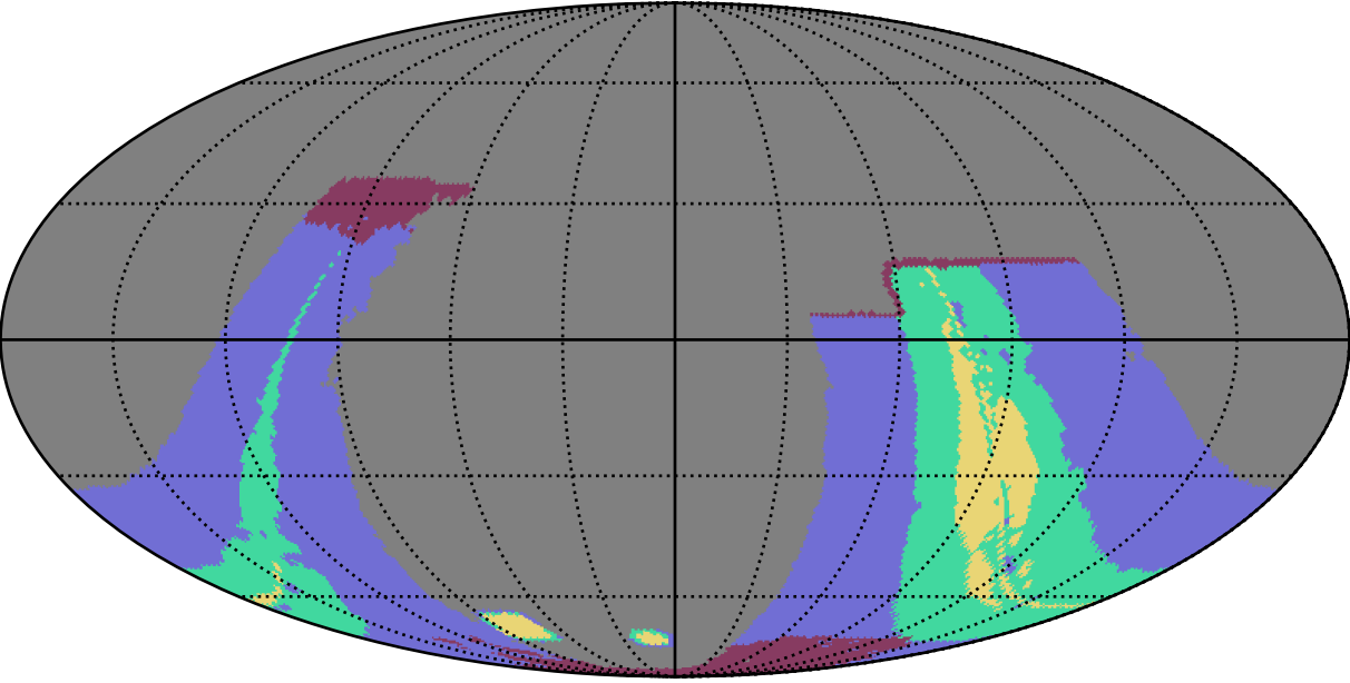
early_ss_template_fpextra1.5_v3.4_10yrs : GalplaneFootprintMetric_galactic_plane_map_Tau_46_5
