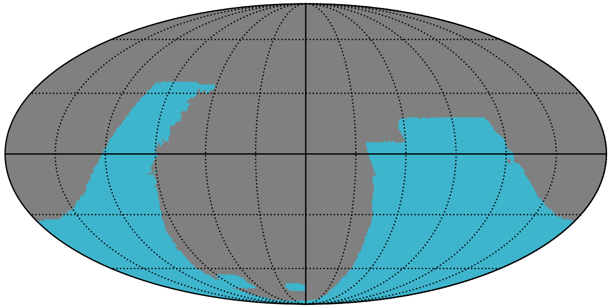
early_ss_template_fpextra1.5_v3.4_10yrs : GalplaneFootprintMetric_galactic_plane_map_Tau_2_0
