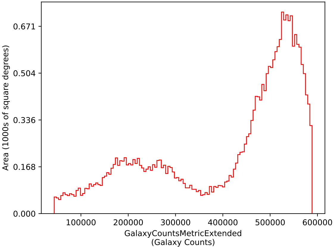
early_ss_template_fpextra1.5_v3.4_10yrs i: GalaxyCountsMetricExtended
