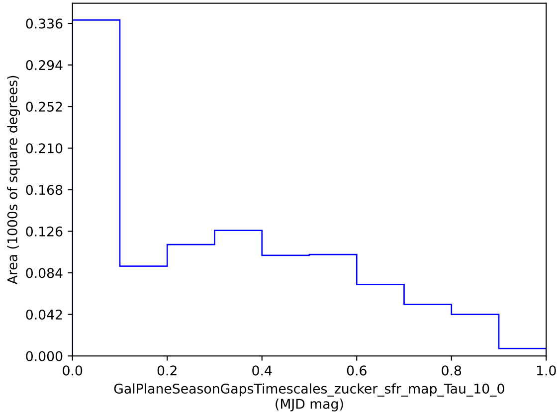
early_ss_template_fpextra1.5_v3.4_10yrs : GalPlaneSeasonGapsTimescales_zucker_sfr_map_Tau_10_0
