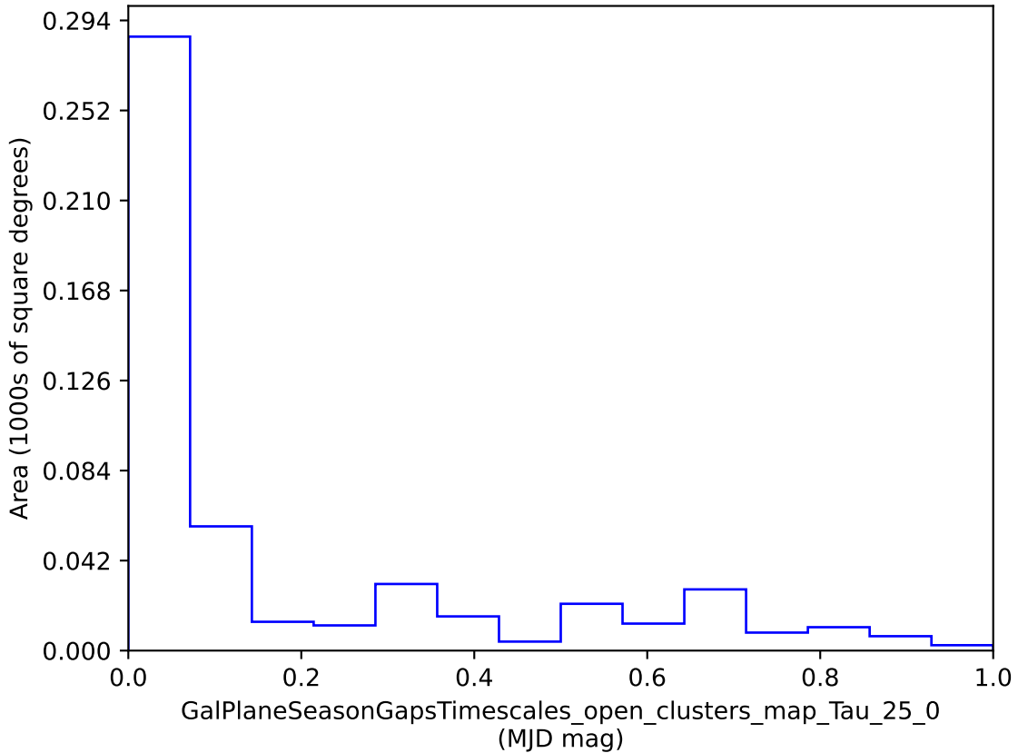
early_ss_template_fpextra1.5_v3.4_10yrs : GalPlaneSeasonGapsTimescales_open_clusters_map_Tau_25_0
