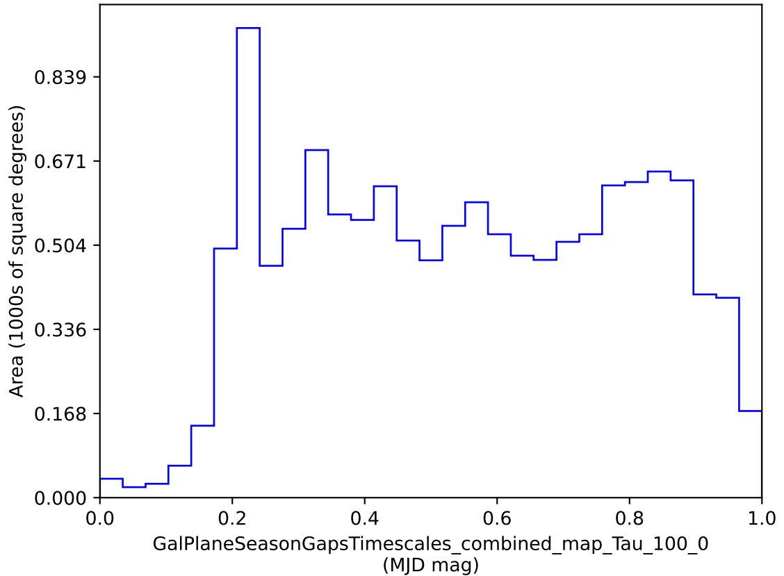
early_ss_template_fpextra1.5_v3.4_10yrs : GalPlaneSeasonGapsTimescales_combined_map_Tau_100_0
