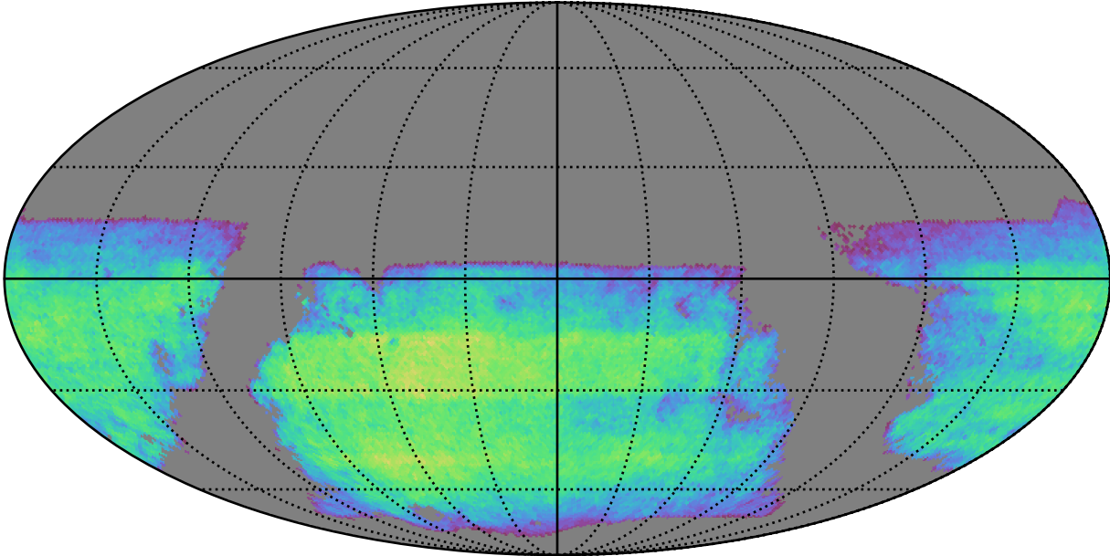
early_ss_template_fpextra1.5_v3.4_10yrs i band non-DD year 7: ExgalM5WithCuts
